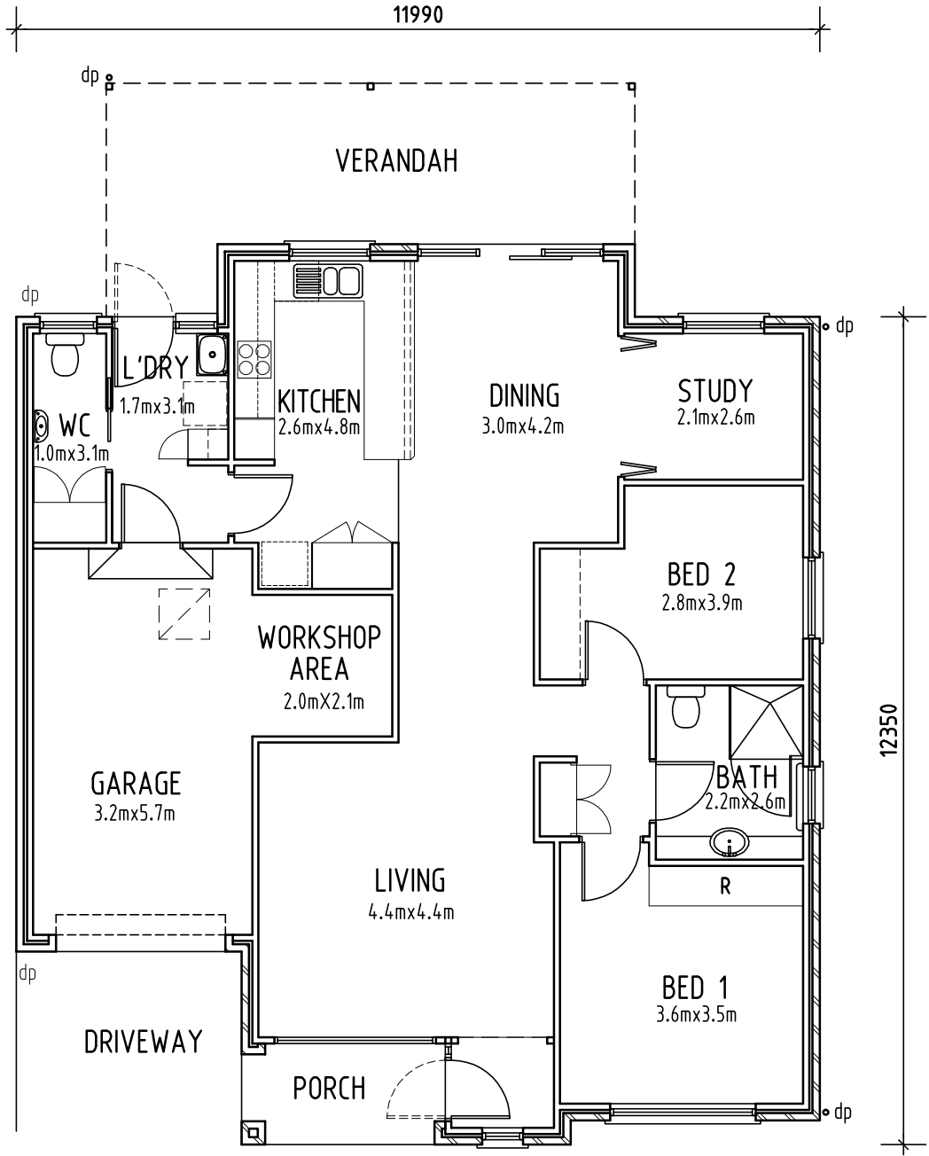
FLOOR PLAN
