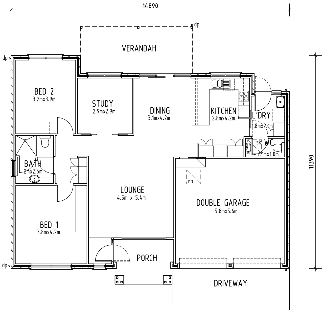
FLOOR PLAN
